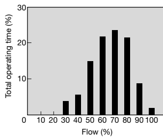
Fig 26 Typical centrifugal pump duty cycle
