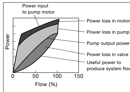
Fig 23 Power consumption in fixed speed pumping
