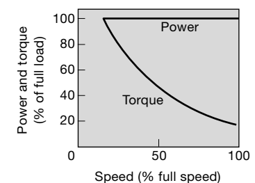
Fig 14 Constant power load
