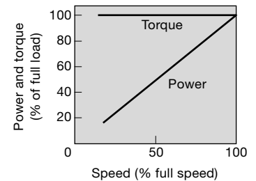
Fig 13 Constant torque load
