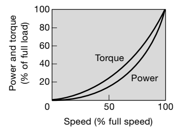
Fig 12 Variable torque load
