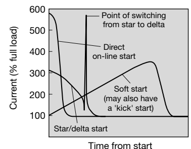
Fig 36 A comparison of current profiles during starting by star/delta, direct-on-line and soft starting
